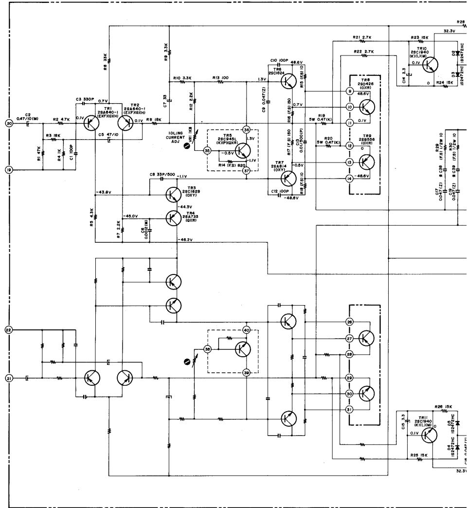
MAIN AMP P.C BOARD M2-5432
