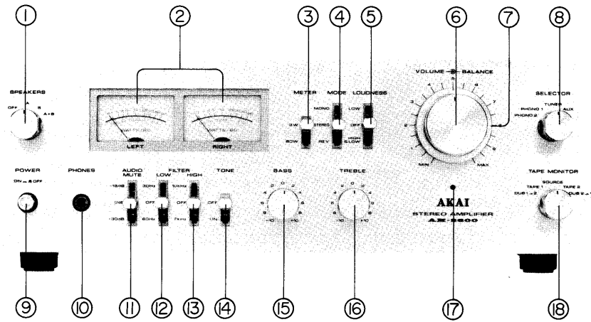
Fig. 1 Controls
