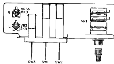
Fig. 7 Volume P.C Board M2-5619
