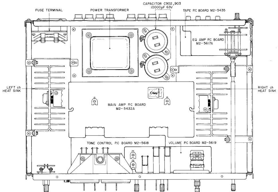
Fig. 2 Top View
