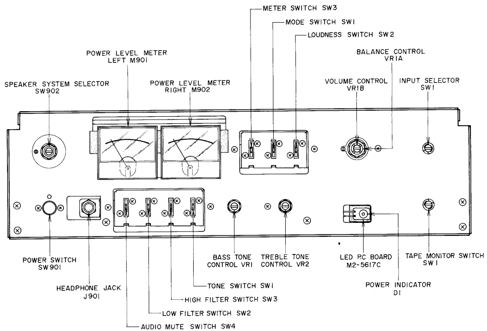
Fig. 3 Front View
